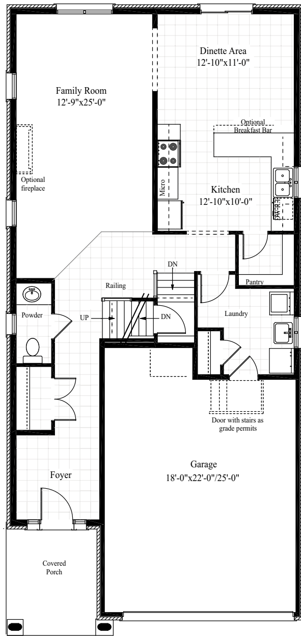
MAIN FLOOR
