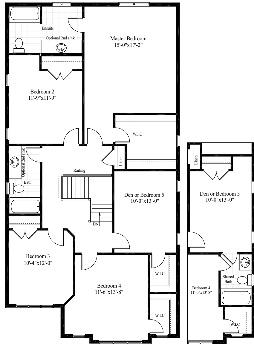
SECOND FLOOR
