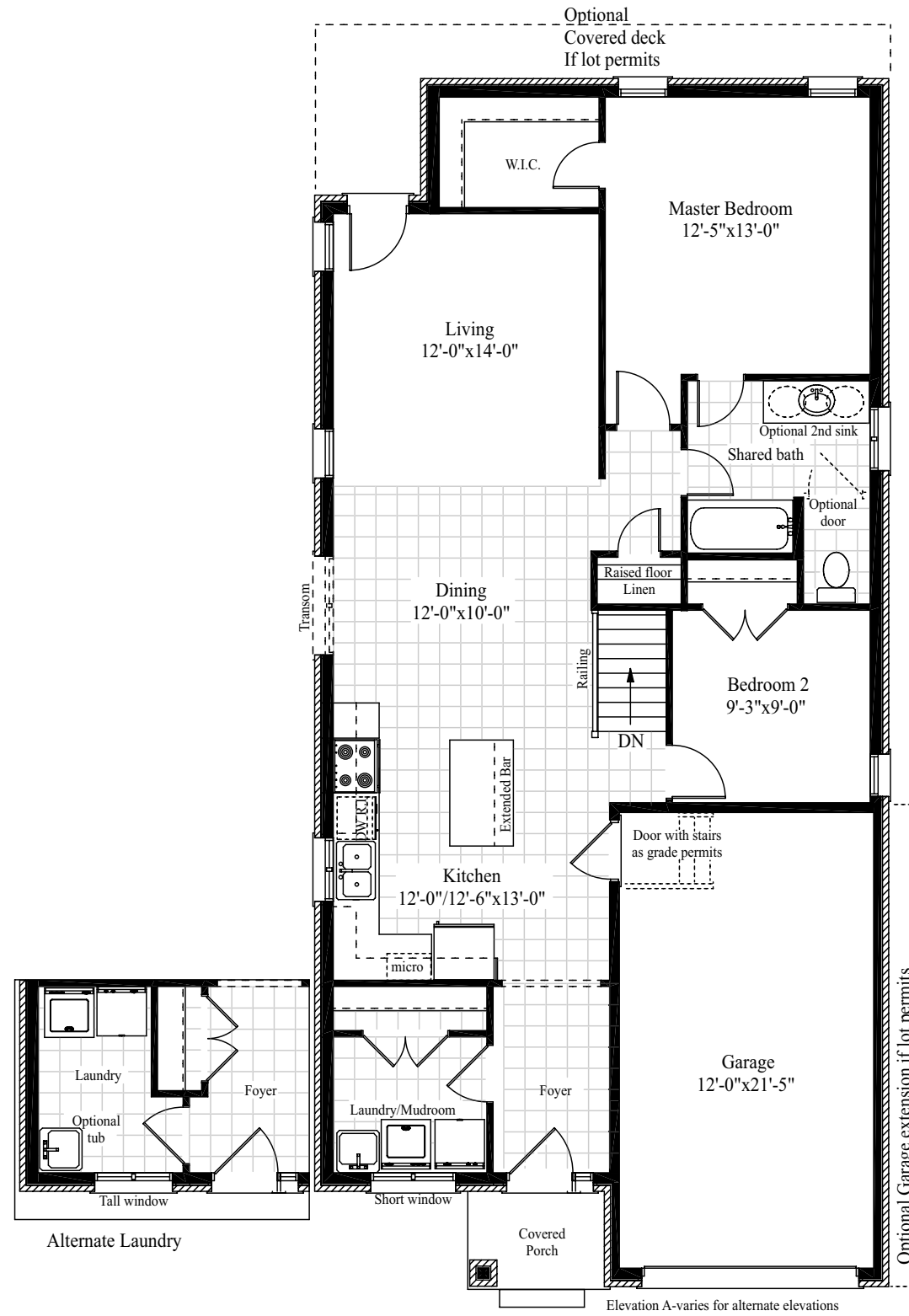
First Floor
