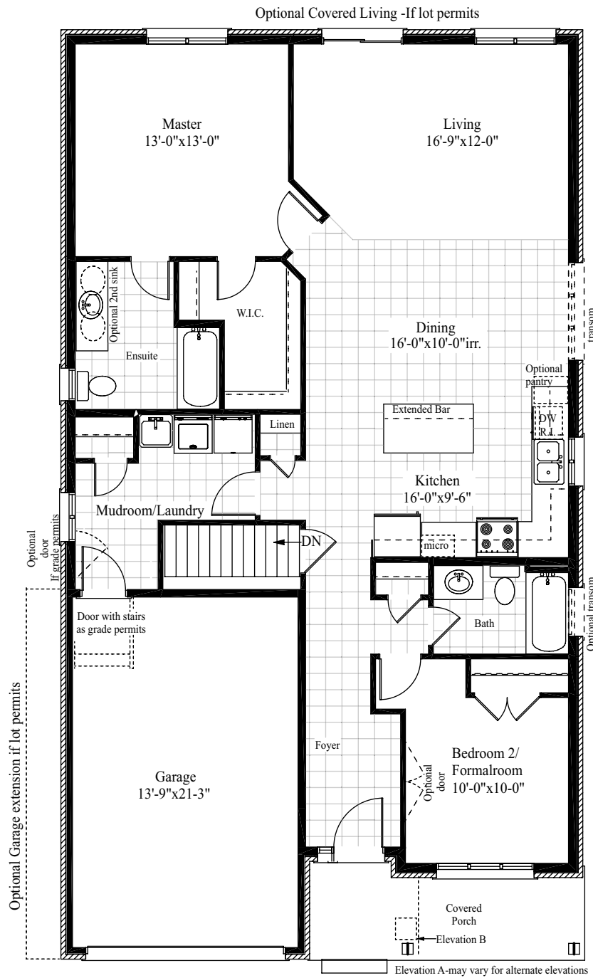
First Floor
