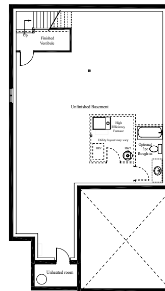
Basement Plan 2/3
