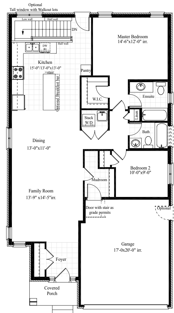
First Floor Plan 3
