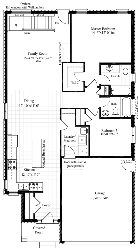
First Floor Plan 2
