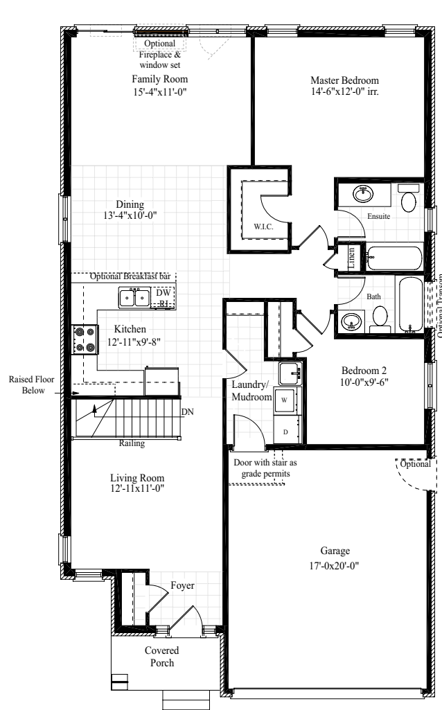
First Floor Plan 1
