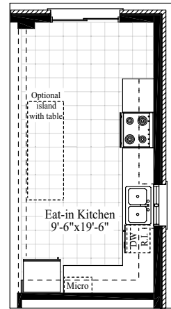
Optional kitchen layout
