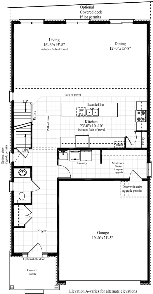
Elevation A-varies for alternate elevations
