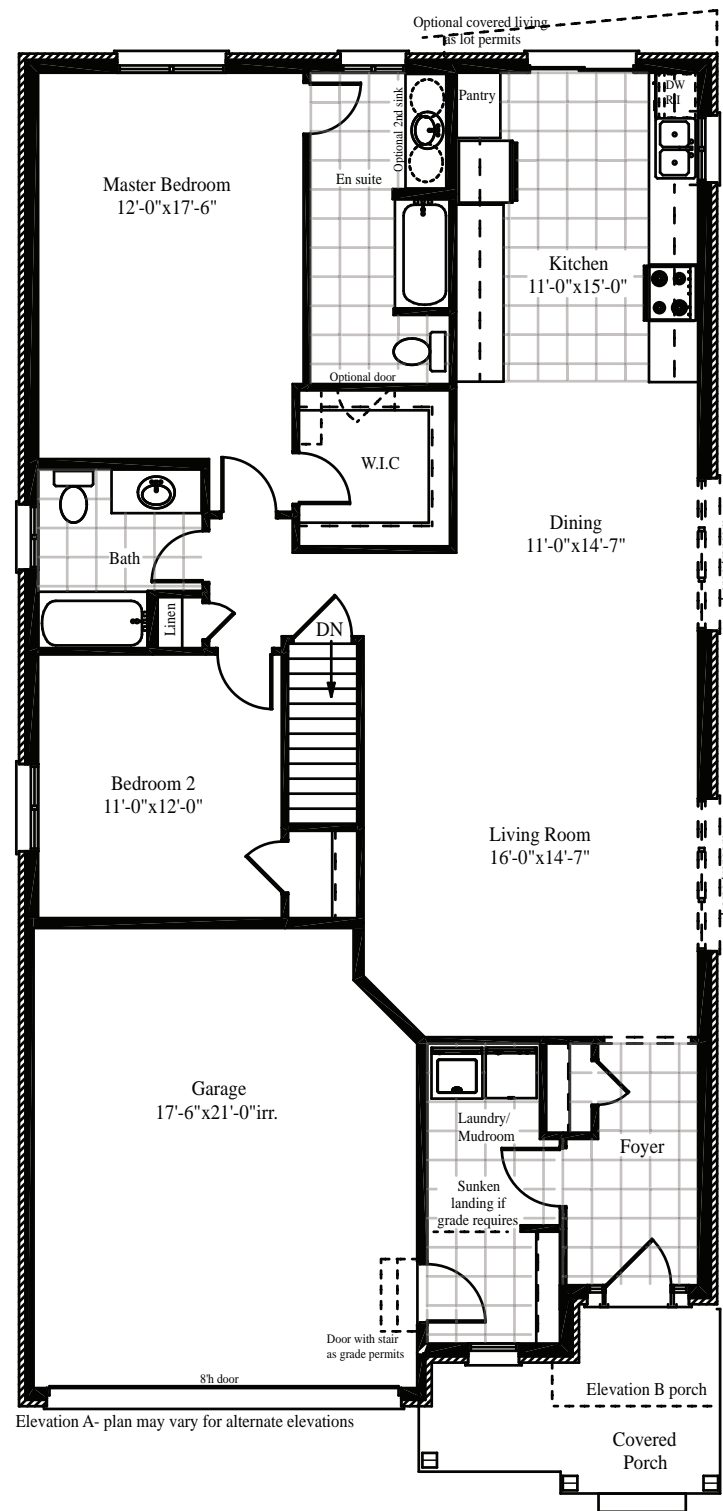
First Floor
