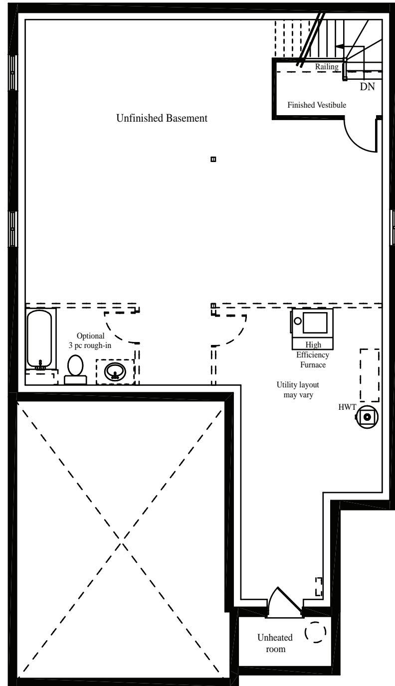
Elevation A- plan may vary for alternate elevations
